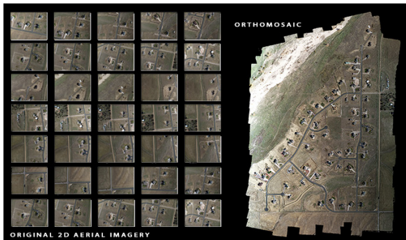
Figure 11: Photogrammetry imagery and a composite image obtained using a UAV.
