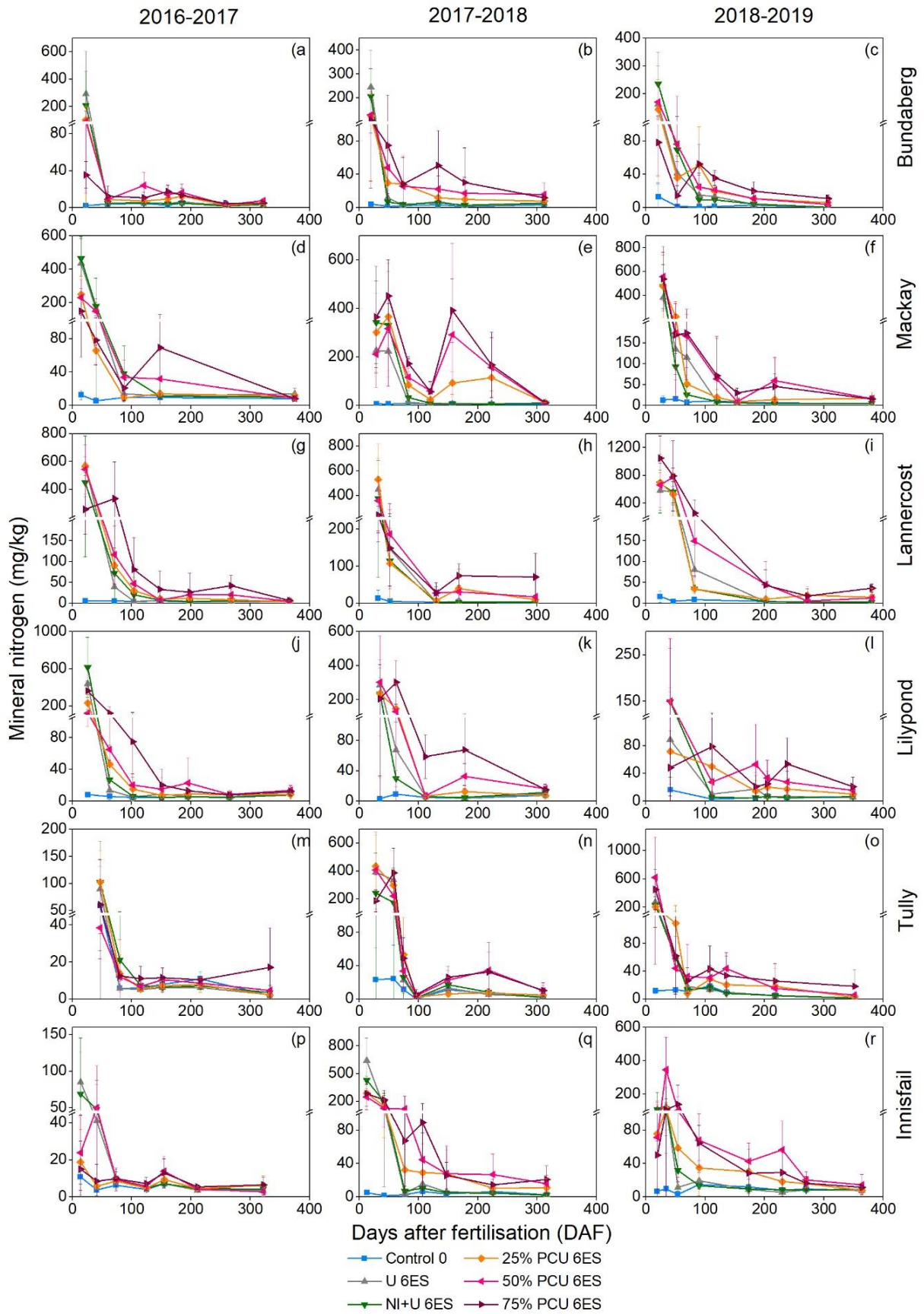
Figure 10. Dynamics of mineral N contents in the 0-20 cm soil after application of different forms of fertiliser at the recommended 6ES rate. The error bars are standard deviations.
