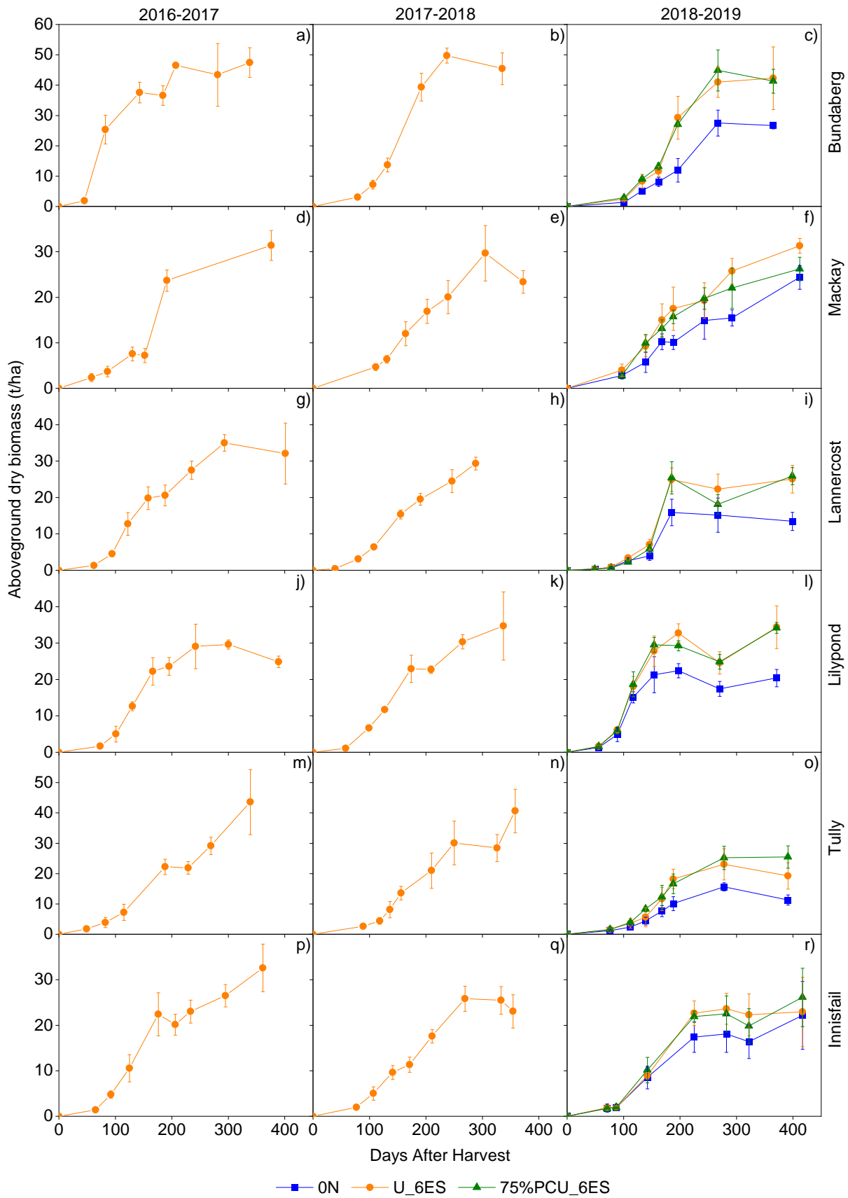
Supp. Figure 2. Dynamics of aboveground plant biomass in selected treatments. See Table 3 for the 6ES rates at each site. The error bars are standard deviations.
