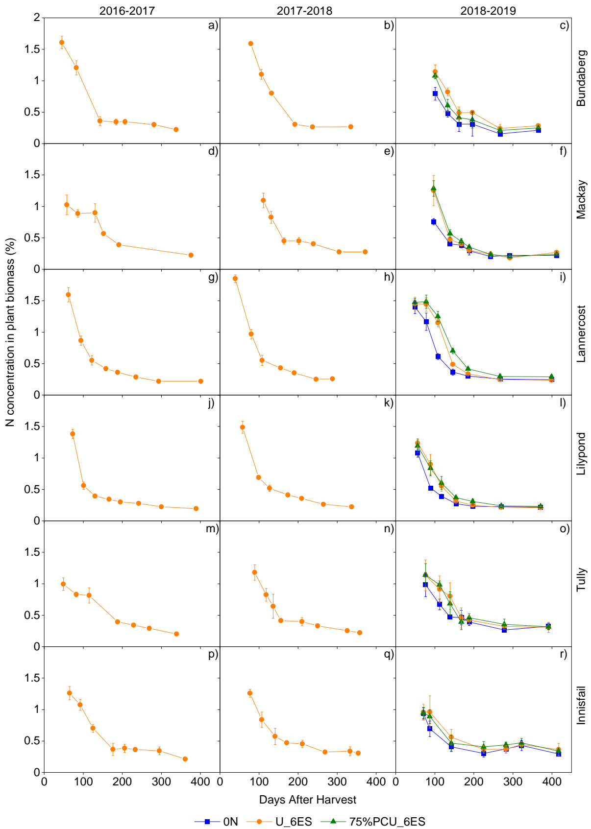
Supp. Figure 3. Dynamics of N contents in the aboveground plant biomass in selected treatments. See Table 3 for the 6ES rates at each site. The error bars are standard deviations.
