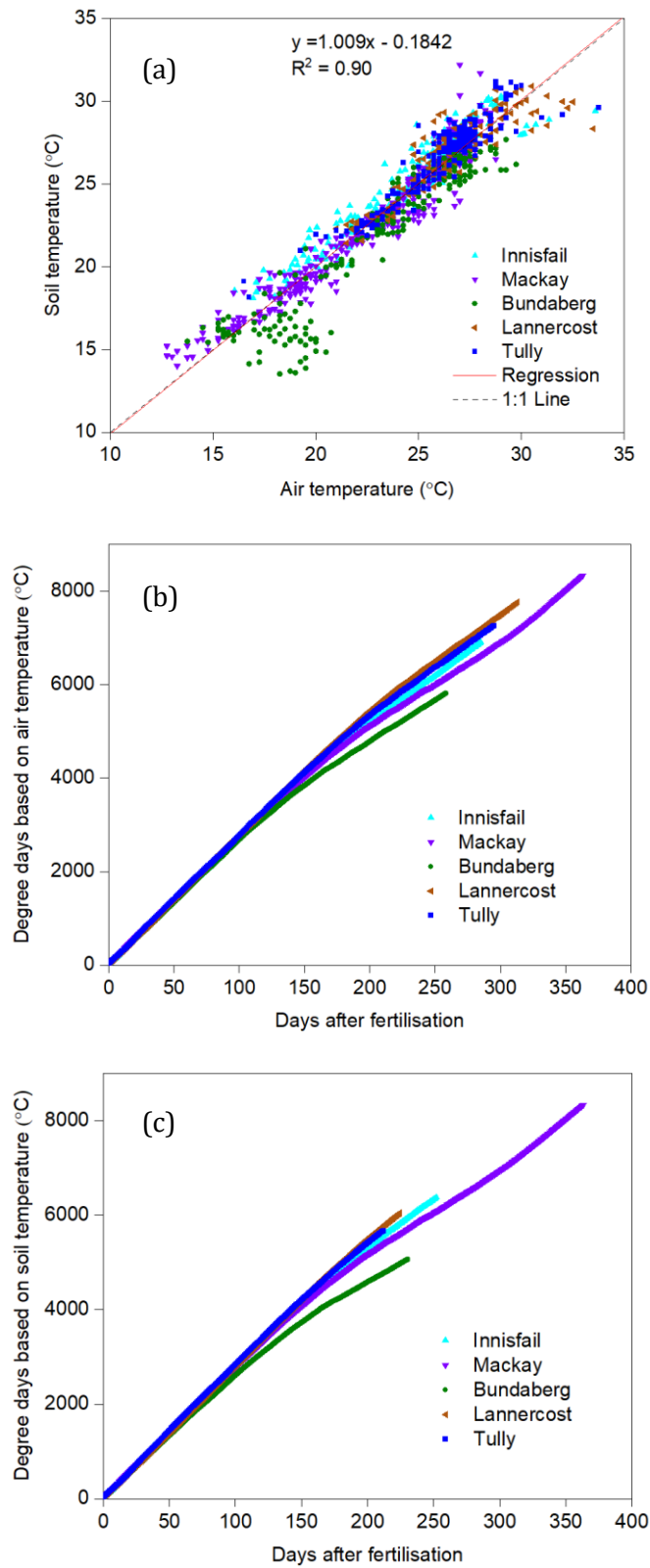
Supp. Figure 1. Similarity between daily soil temperature at a depth of 10 cm and air temperature and between degree days calculated with air and soil temperature in the 2018-19 season.
