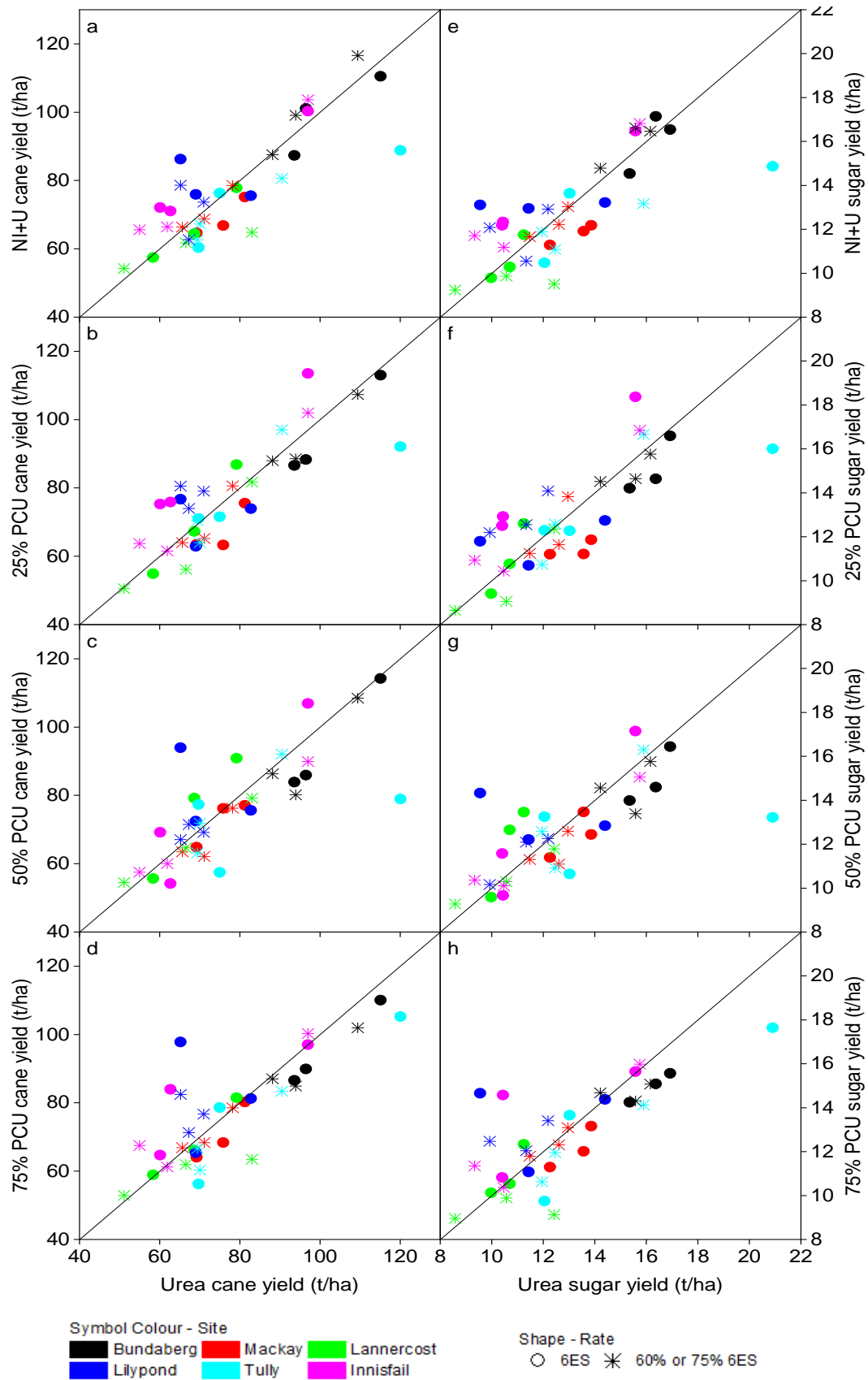
Suppl. Figure 5. Comparison of cane (a-d) and sugar (e-h) yield responses to EEFs vs. standard urea at the same N application rate. See Table 3 for the 6ES rate at each site.
