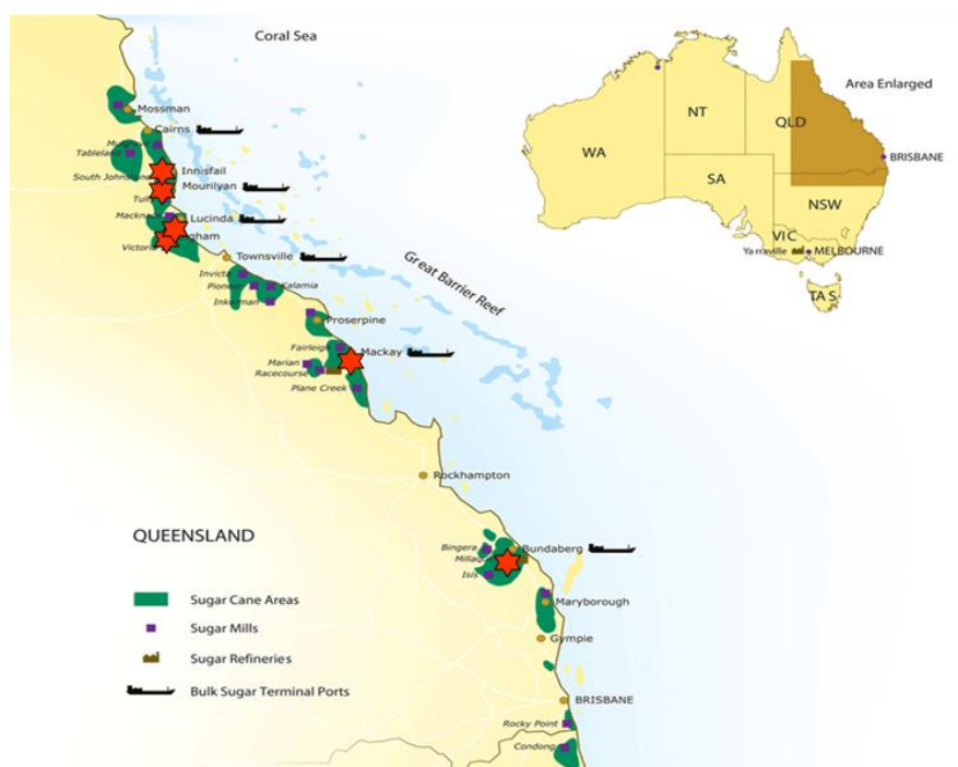
Figure 1. Location of the field trials (indicated by red stars). The map was adapted with permission from the Queensland Cane Growers Organisation (2020).
